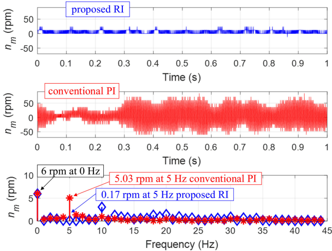
Fig. 15. Tracking 6 r/min against inertia variation ( J = 0.5 \cdot 10^{-3} \text{ kg}\cdot\text{m}^2 ). Time waveforms and their FFTs (proposed RI in blue and conventional PI in red).
